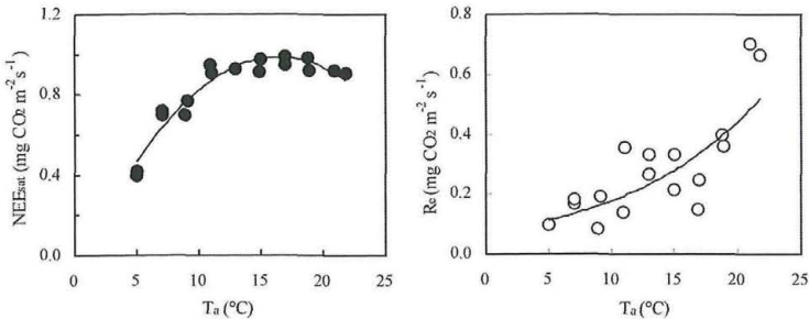
Fig. 4. Relationship between light-saturated net ecosystem exchange ( NEE_{sat} ) and air temperature ( T_a ) (left) and relationship between dark respiration ( R_e ) and air temperature ( T_a ) (right) in growth period for two years. Regression line is NEE_{sat} = -0.004T_a^2 + 0.1308T_a - 0.0901 ; r^2 = 0.93 and R_e = 0.0706e^{0.0917T_a} ; r^2 = 0.65 , respectively.
