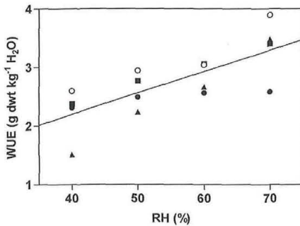
Fig. 3. Linear relationship between plant water use efficiency (WUE) and relative air humidity (RH) of four Chinese conifer tree species ( \blacktriangle , P. massoniana ; \blacksquare , P. tabulaeformis ; \circ , P. orientalis ; \bullet , C. lanceolata ). Data represent the integrated WUE measured on 12 plants. The line represents the linear relationship between WUE and RH for the four species. The equation for the line is; WUE = 0.0365RH + 0.74 , R^2 = 0.56 , P = 0.001 .
