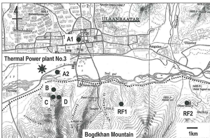
Fig. 1. Locations of the monitoring sites. Sites A1 and A2 were at the Ulaanbaatar Monitoring Station and the CLEM compound, respectively. Sites B, C and D were in a boundary area between grassland, an open forest and a closed forest, respectively. Sites RF1 and RF2 were at certain distance from the power plant as reference forest areas. Sites A1, RF1 and RF2 were newly added in 2003, while site D was surveyed only in 2001.
