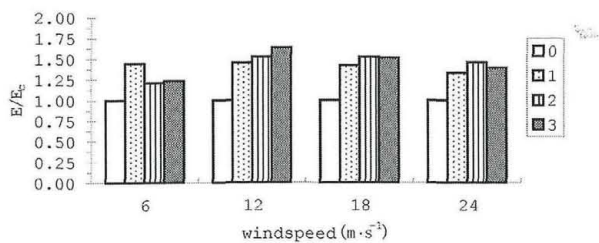
Fig. 1. Transpiration rate (E) dependent on wind speed and exposure events. E/Ec is the ratio of exposed plant to control one, and 0, 1, 2 or 3 represents the number of exposure events.
