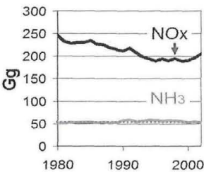
Fig. 1. Emissions of NO x and NH 3 in Austria (Gg p.a.; Umweltbundesamt 2002)
