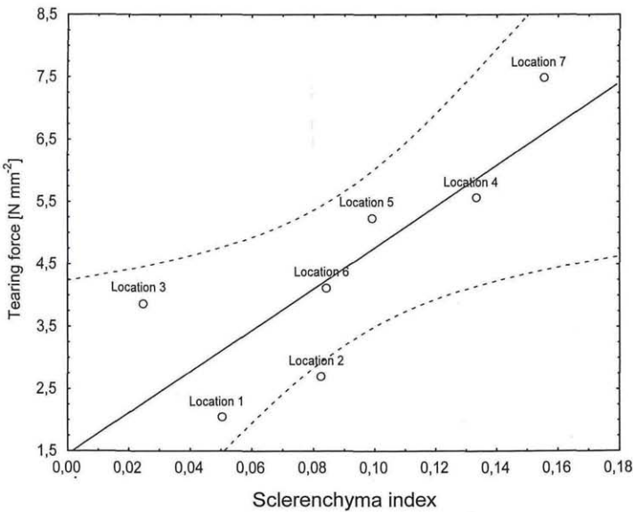
Fig. 3. Correlation between sclerenchyma index and tearing force needed to break the stem. The measurements were done using „ZWICK ZO507TH3A“ apparatus. (N = 4 per growing site; solid line ÷ regression; dotted line ÷ 95% confidence interval)
