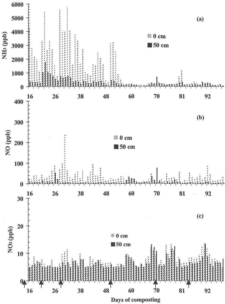
Fig. 4. Concentration of NH 3 , NO and NO 2 at 0 and 50 cm above the windrow surface under active aeration treatment (arrows pointing to data of windrow turning).
