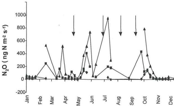
Fig. 3. Seasonal \text{N}_2\text{O} fluxes from grazed grassland: preliminary data from grass-clover (◆) or undrained (■) or drained (▲) grass (receiving c. 280 \text{ kg N ha}^{-1} \text{ y}^{-1} ) swards. Arrows denote times of fertilizer application. (YAMULKI, unpublished information)
