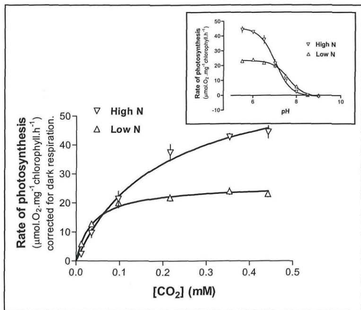
Fig. 4. Light induced O_2 evolution of E. canadensis leaves at 60 \mu\text{mol m}^{-2} \text{s}^{-1} versus [CO_2] , [DIC] was constant, 1 mM. [CO_2] was varied by changing the pH, see inset.
