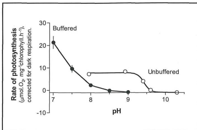
Fig. 1. Light induced O_2 production rate, corrected for dark respiration, of E. canadensis leaves plotted against pH using either a strongly buffered (25 mM MES/BTP) or an unbuffered APW solution containing 1 mM HCO_3^- .
