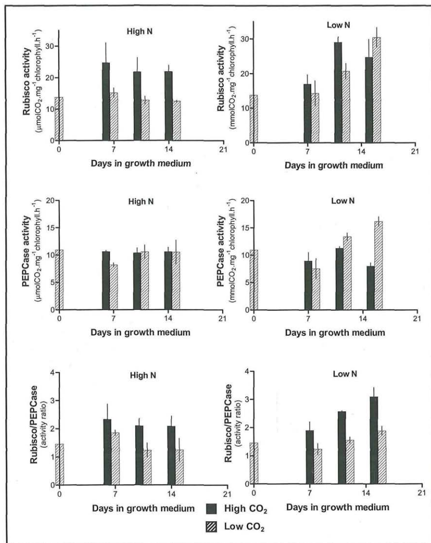
Fig. 3. Rubisco and PEPCase activity of E. canadensis shoots grown in 5% Hoagland solution for 1-2 weeks, at high or low N and low or high CO 2 , fluence rate 60 \mu\text{mol m}^{-2} \text{s}^{-1} PAR, photoperiod 12 h, 21 °C. 1-2 weeks.
