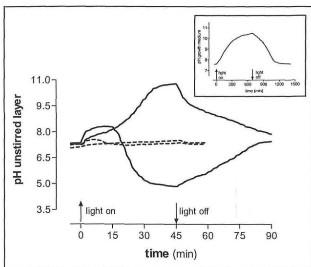
Fig. 2. pH-polar reaction of E. canadensis leaves grown at either low or high \text{CO}_2 . Medium: 5% Hoagland low N, fluence rate 60 \mu\text{mol m}^{-2} \text{s}^{-1} PAR. Inset: Culture solution pH of low \text{CO}_2 culture, one light-dark cycle (24 hours).
