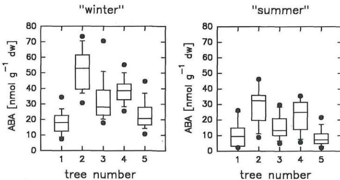
Fig. 1. Box plot of ABA concentrations during "winter" (23.11.94 - 21.04.95) and "summer" (18.05.95 - 11.10.95) of five Pinus cembra trees. Box displays the 25 th , 50 th and 75 th percentile, marks represent the 10 th and 90 th percentile.
