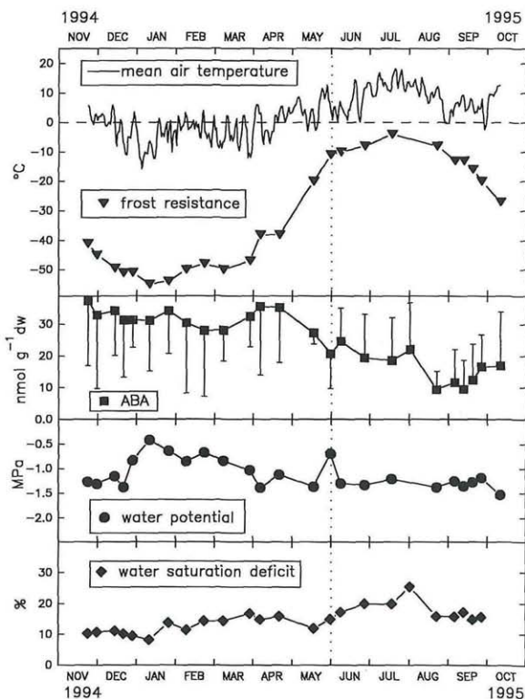
Fig. 2. Mean seasonal variation of the ABA concentration of five Pinus cembra trees, and of frost resistance, water potential and water saturation deficit in needles formed in 1994 as compared with the seasonal course of the air temperature. Bars indicate SD ( n=5 ), broken line indicates budbreak.
