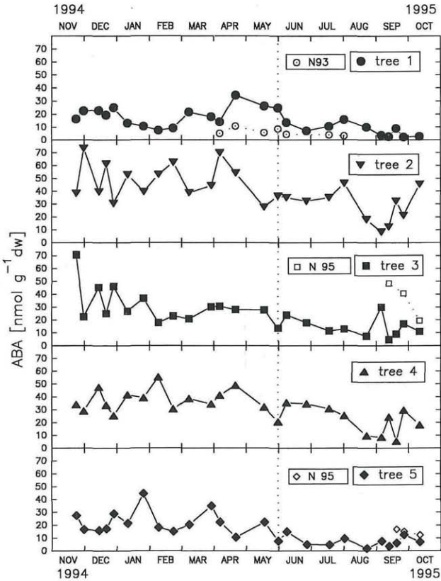
Fig. 3. Seasonal variation of ABA level in needles formed in 1994 for five Pinus cembra trees. ABA concentration in needles formed in 1993 and 1995 is added for selected sampling dates for trees 1, 3 & 5. Broken line indicates budbreak.
