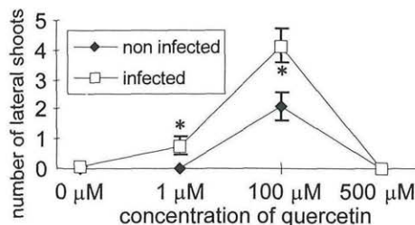
Fig. 4. Number of lateral shoots of healthy and PVY NTN infected plants grown on media containing 0, 1, 100 or 500 µM of quercetin after 8 weeks. At values indicated with star, the infected plants significantly differ from the non infected plants ( p < 0.05 ). Standard errors are indicated by error bars.
