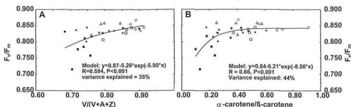
Fig. 3. Correlations between carotenoid composition and chlorophyll fluorescence. \bullet , \circ site I, \blacklozenge , \diamond site II, \blacksquare site III, \blacktriangle , \triangle site IV. Open symbols = current year's needles, filled symbols = one year old needles. A. State of the xanthophyll cycle versus F_v/F_m . V = Violaxanthin, A = Antheraxanthin, Z = Zeaxanthin. B. \alpha -Carotene/ \beta -Carotene ratios versus F_v/F_m .
