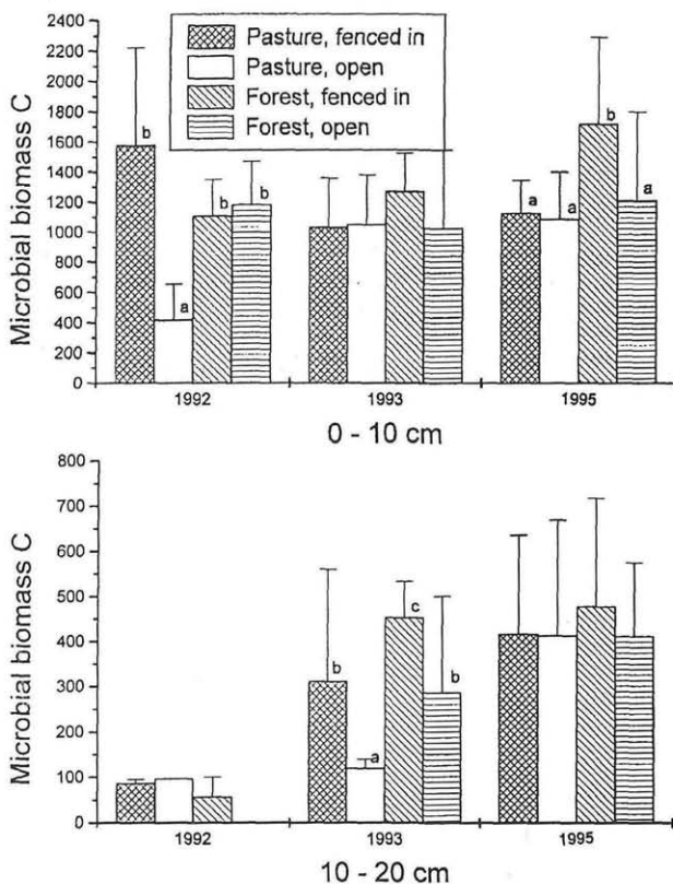
Fig. 2. Biomass [ \mu\text{g C}_{\text{mic}} \text{g}^{-1} soil] for the soils sampled in 1992, 1993 and 1995 (Mean \pm standard deviation). Different letters (a, b, c) indicate significant ( P < 0.05 ) differences between treatments within one year. Above: upper horizon (0-10 cm), below: lower horizon (10-20 cm).
