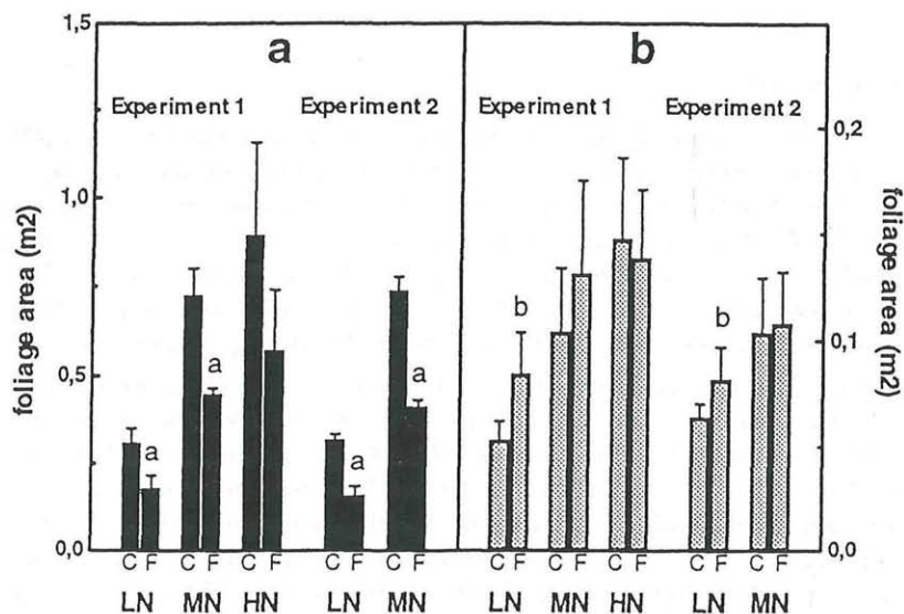
Fig. 2: Foliage area of a) foliage of the whole tree and b) foliage younger than four weeks developed on the main stem. C = control; F = fumigated with ozone.
