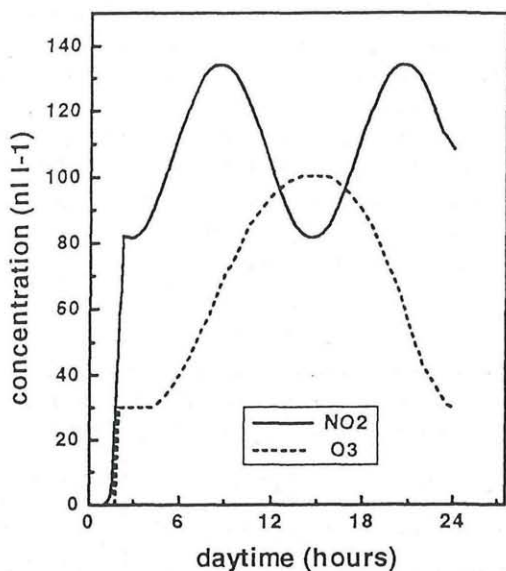
Fig. 1: Daily course of ozone and \text{NO}_2 concentrations during the fumigation experiments. Mean concentrations: 60 \text{ nl l}^{-1} ozone and 100 \text{ nl l}^{-1} \text{NO}_2 .
