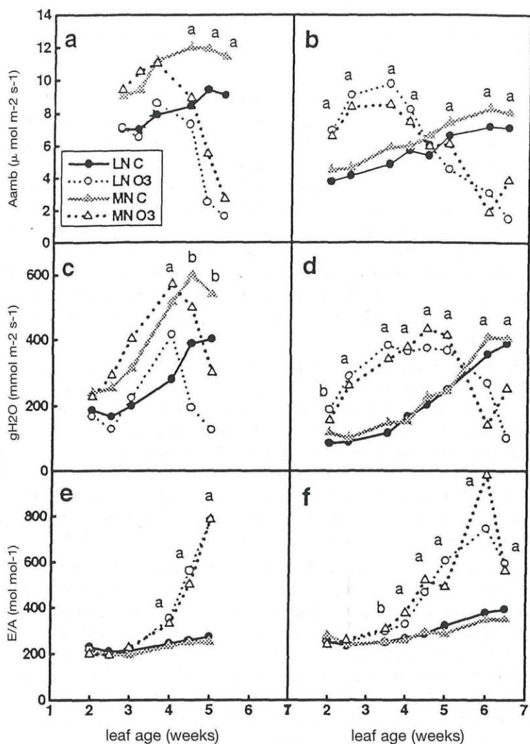
Fig. 3: a) and b) net \text{CO}_2 assimilation rate at ambient \text{CO}_2 concentrations (Aamb); c) and d) stomatal conductance ( g_{\text{H}_2\text{O}} ); and e) and f) transpiration rate by Aamb (E/A); of the leaves along the main stem profile, determined after 9 (a, c, e) and 15 (b, d, f) weeks of exposure. Mean values (5 replicates) for LN control (LN C), LN ozone (LN \text{O}_3 ), MN control (MN C) and MN ozone (MN \text{O}_3 ). Statistical significance of fumigation effect (multifactor ANOVA) p < 0.01 = a ; p < 0.05 = b . Significant fertilization effects were found for Aamb and g_{\text{H}_2\text{O}} after 9 weeks of exposure (p values not shown).
