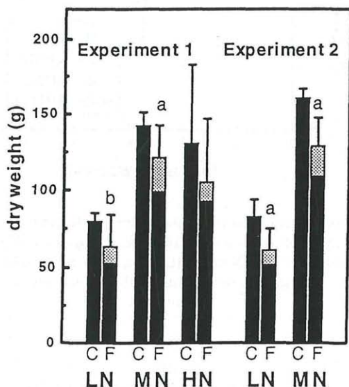
Fig. 5: Whole-plant biomass after 12 weeks of exposure (black) and total biomass of shed leaves (gray). C = control, F = fumigated with ozone. Mean values (columns) and error bars ( n = 5 ). Statistical significance of fumigation effect (Kruskal-Wallis) p < 0.01 = a ; p < 0.05 = b (indicated values for biomass without shed leaves).
