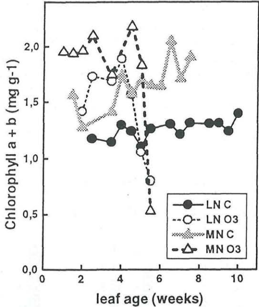
Fig. 4: Total chlorophyll concentrations (i.e. chlorophyll a and b) of the leaves along the main stem profile, determined after 16 weeks of exposure. Mean values (5 replicates) for LN control (LN C), LN ozone (LN O 3 ), MN control (MN C) and MN ozone (MN O 3 ). For statistical significance of fumigation effect refer to text. Data for experiment 2.
