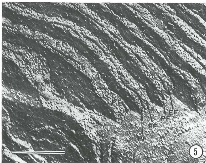
Figs. 4, 5. Freeze-fractured thylakoid membranes of Callithamnion caudatum (Fig. 4) and Polysiphonia deusta (Fig. 5). Randomly distributed particles are seen on both EF and PF in the two species; in Callithamnion caudatum tend to be organized into rows (arrows). (EF and PF see Fig. 2.) Fig. 4, x 125,000; Fig. 5, x 100,000.
