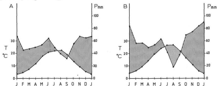
Fig. 2. Ombrothermic diagrams of the two meteorological stations, A: Chrysopigi and B: Drama.
