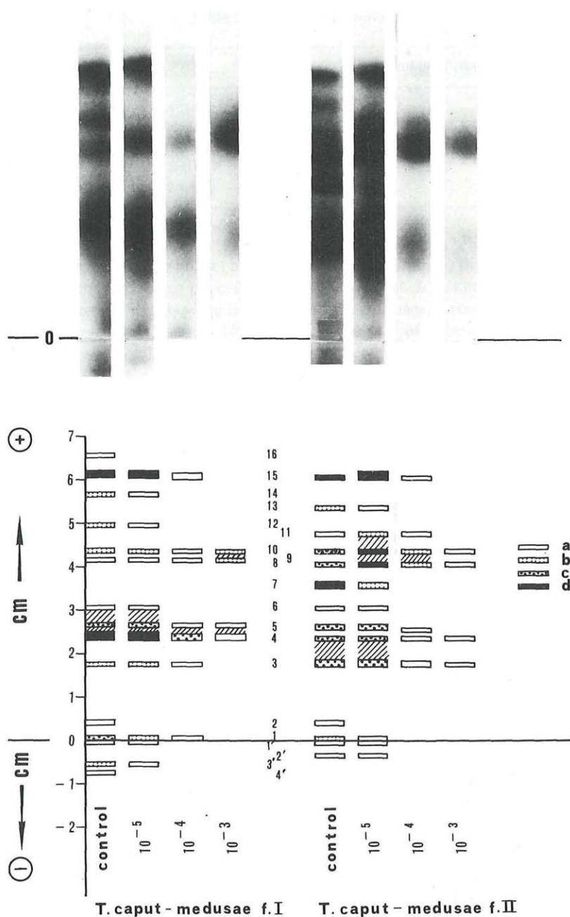
Fig. 1. Effects of dibrom on shoot esterase patterns of T. caput-medusae form I and form II. Photograph and corresponding schematic representation. On the right: key to shading in order of increasing band intensities.
