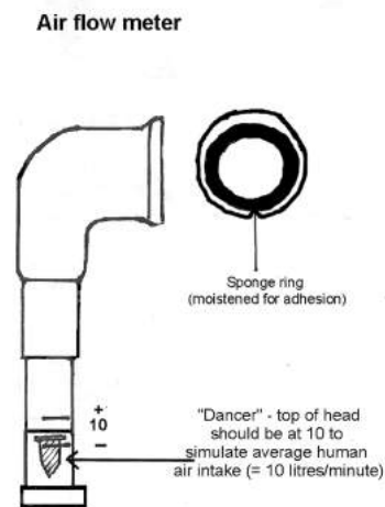
Figure 2. Diagram of the air flow meter used.
