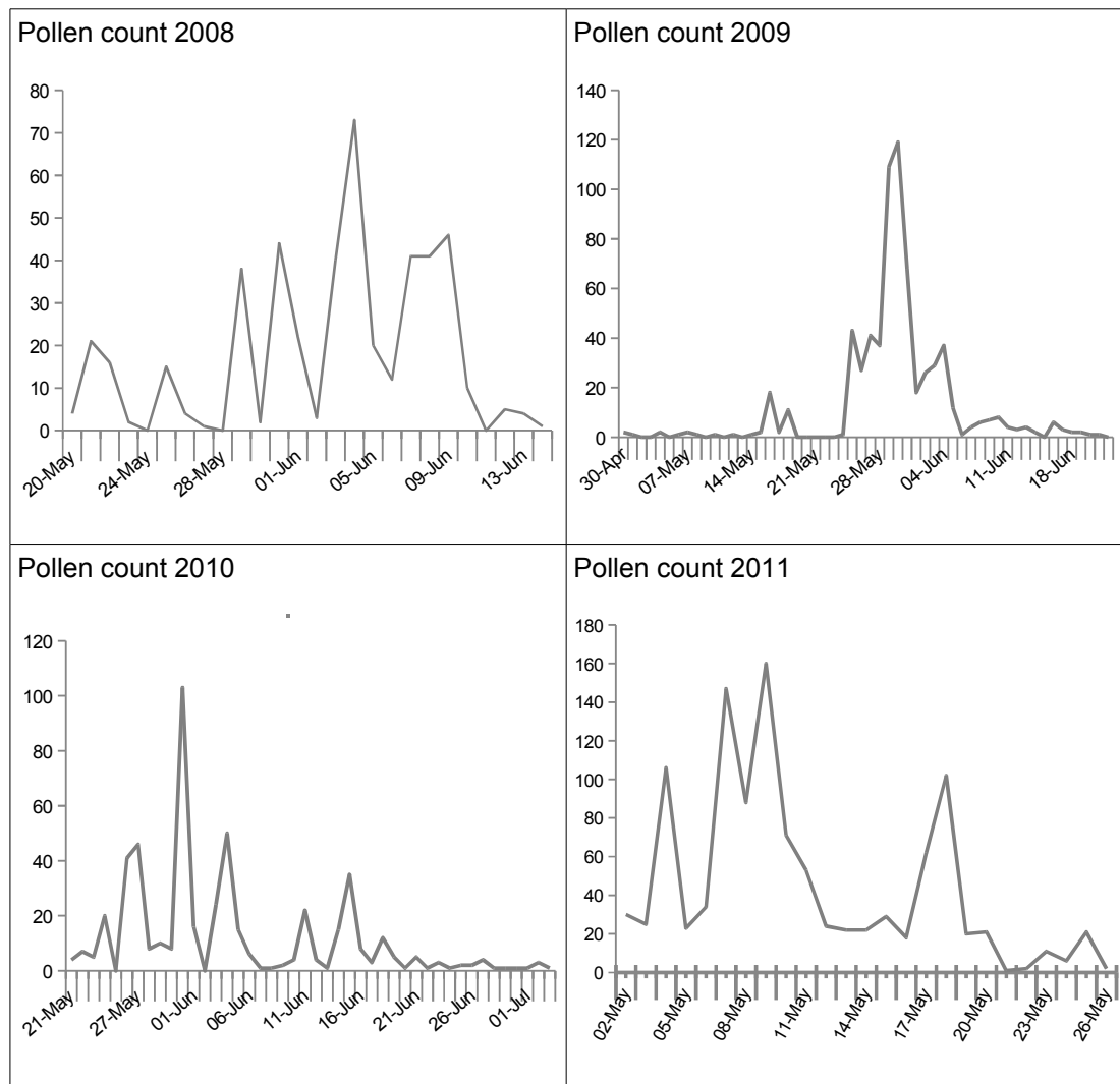
Figure 4. Graphs of pollen counts 2008-2011. The counts (y-axis) are in pollen grain numbers per cubic metre of air sampled (pgs/m 3 air).
