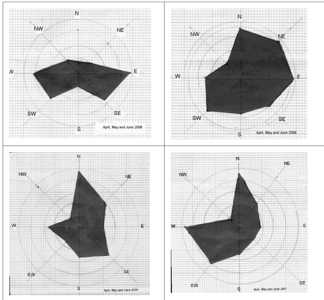
Figure 3. Wind roses for the months of April, May and June for the years 2008 (top left), 2009 (top right), 2010 (bottom left) and 2011 (bottom right).
