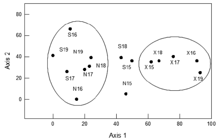
Figure 8. Ordination plot for ground flora in the Upper Burbage Valley enclosure and in the control area outside the enclosure. N15-N19 represent the northern half of the enclosure in 2015-2019, S15-19 represent the southern half of the enclosure in 2015-2019, and X15-19 represent the control area in 2015-2019. Points that are closer together have greater similarity of ground flora.
