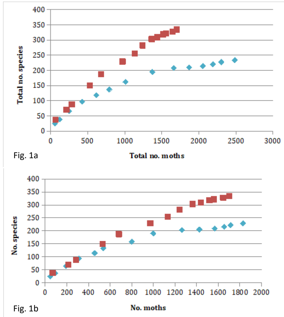
Fig. 1. (a) Species accumulation curves for Askham Bog (squares) and a suburban garden in Huntington (diamonds); (b) the same data but omitting the five most abundant species in the garden site, viz. Agrotis exclamationis , Noctua pronuba , Xestia xanthographa , Apamea monoglypha and Hoplodrina octogenaria . The two sites are 6 miles apart and data are for the 14 nights in 2020 when an MV trap was operated at each site. It is possible to fit a power function regression to these data (giving lines of best fit as y=1.68x^{0.72} for Askham Bog and y=2.34x^{0.60} for Huntington Road, confirming the differences between the two sites; however, as stated in the text, deviations from this fit at high values of x mean that such an approach cannot be used predictively.
