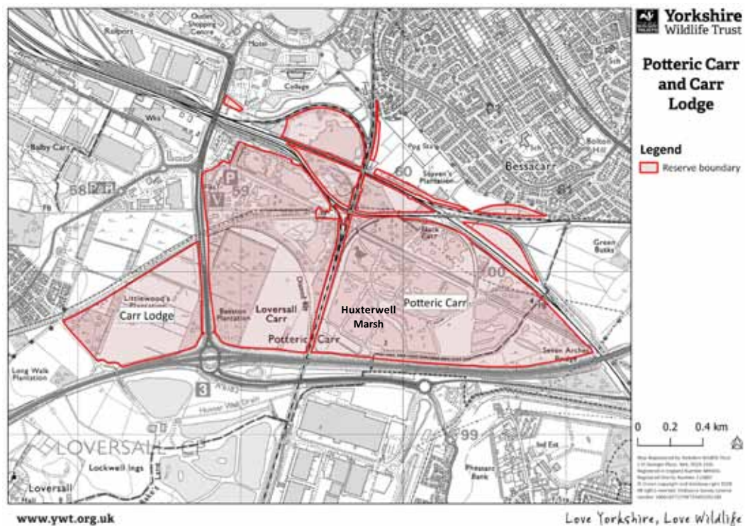
Figure 1. Potteric Carr and Carr Lodge nature reserves shown with red line.
