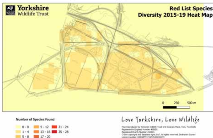
Figure 3. Heat map of red listed species
