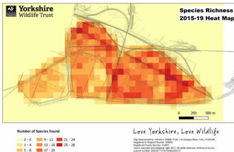
Figure 5. Map showing species richness
