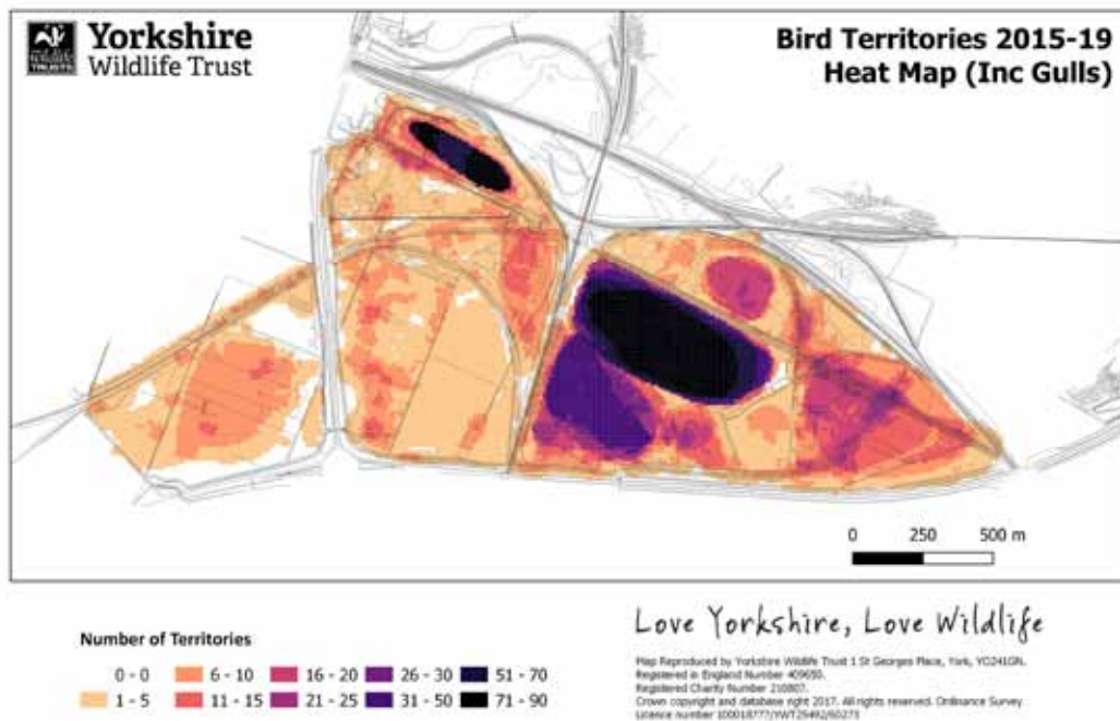
Figure 2. Heat map of territories of all birds.
