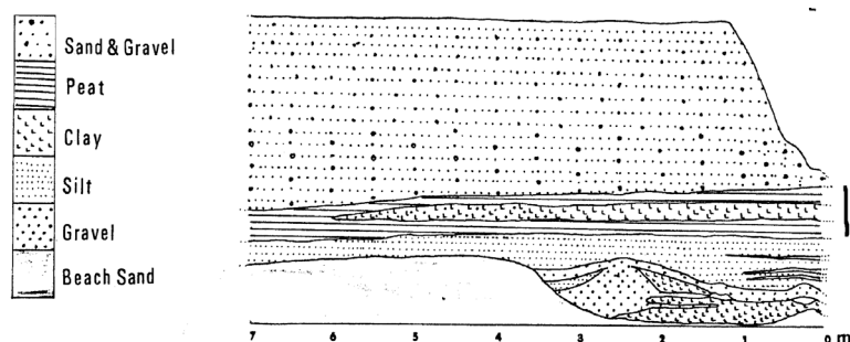
Figure 2. West-east section on the north side of the Barmston Drain, east of Horse Bridge, recorded in 1980 (JDA).
