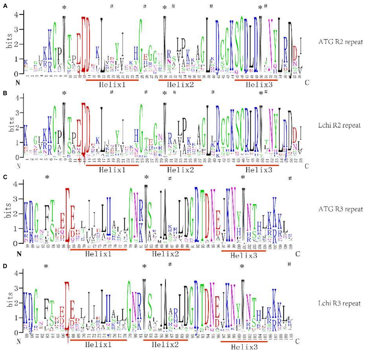
FIGURE 1 | Sequence logos of the R2 and R3 MYB repeats from Liriodendron chinense ( Lchi ) and Arabidopsis . Multiple sequence alignment analysis of 76 Lchi and 126 Arabidopsis R2R3-MYB domains was used in ClustalX2.1. Panels (A,B) were the R2 repeats, and panels (C,D) were the R3 repeats in Arabidopsis and Lchi . N and C represent the N-terminal and C-terminal, respectively, and the bit score shows the conservative information for all positions in the sequence; the higher the value, the higher the conservation, and the different colors were generated by the website randomly. The asterisks represent the highly conserved tryptophan (W) and phenylalanine (F) residues, and the # represents the different patterns of positions between Lchi and Arabidopsis .
