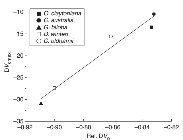
FIG. 4. Relationship ( y = 244x + 192 , r^2 = 0.95 , P = 0.003 ) between the relative observed changes in the in situ oxygenation rate [Rel. DV_O = (V_{\text{Oamb}} - V_{\text{OTJB}})/V_{\text{Oamb}} ] and the corresponding changes in the maximum rate of carboxylation ( DV_{\text{Cmax}} ). DV_{\text{Cmax}} data are differences resulting after subtraction of the mean values of the ambient treatment (400 ppm \text{CO}_2 , 21 % \text{O}_2 ) from the corresponding values of the TJB (1900 ppm \text{CO}_2 , 16 % \text{O}_2 ) treatment.
