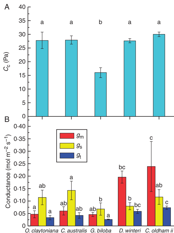
FIG. 2. (A) Operational chloroplastic CO 2 concentrations ( C_c ) of the test species under ambient atmospheric conditions (400 ppm CO 2 , 21 % O 2 ). Data are means ± s.d. from 3–4 measurements. Different letters denote statistically significant differences ( P \leq 0.05 ) between species. (B) Mesophyll conductance ( g_m ), stomatal conductance at saturating light intensity ( g_s ) and total conductance [ g_t = (g_m \times g_s)/(g_m + g_s) ] of the test species under ambient atmospheric conditions (400 ppm CO 2 , 21 % O 2 ). n = 3-4 depending on species. The error bars denote 1 s.d. Different letters for each parameter denote statistically significant differences ( P \leq 0.05 ) between species.
