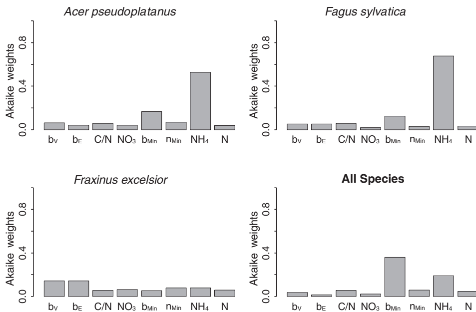
Fig. 3. – Akaike weights for linear mixed effects models relating shoot growth of tree seedlings recorded in 50 \times 50 cm plots in a mixed montane forest in the North-eastern Calcareous Alps to various predictor variables. bV and bE are models with predictor variables soil pH and incoming radiation, or Ellenberg's L and R values, respectively. The other models were bV and bE models that included also one of the soil variables (C:N ratio, NO 3 content, b Min = gross mineralization, n Min = net mineralization or NH 4 content) or Ellenberg's.
