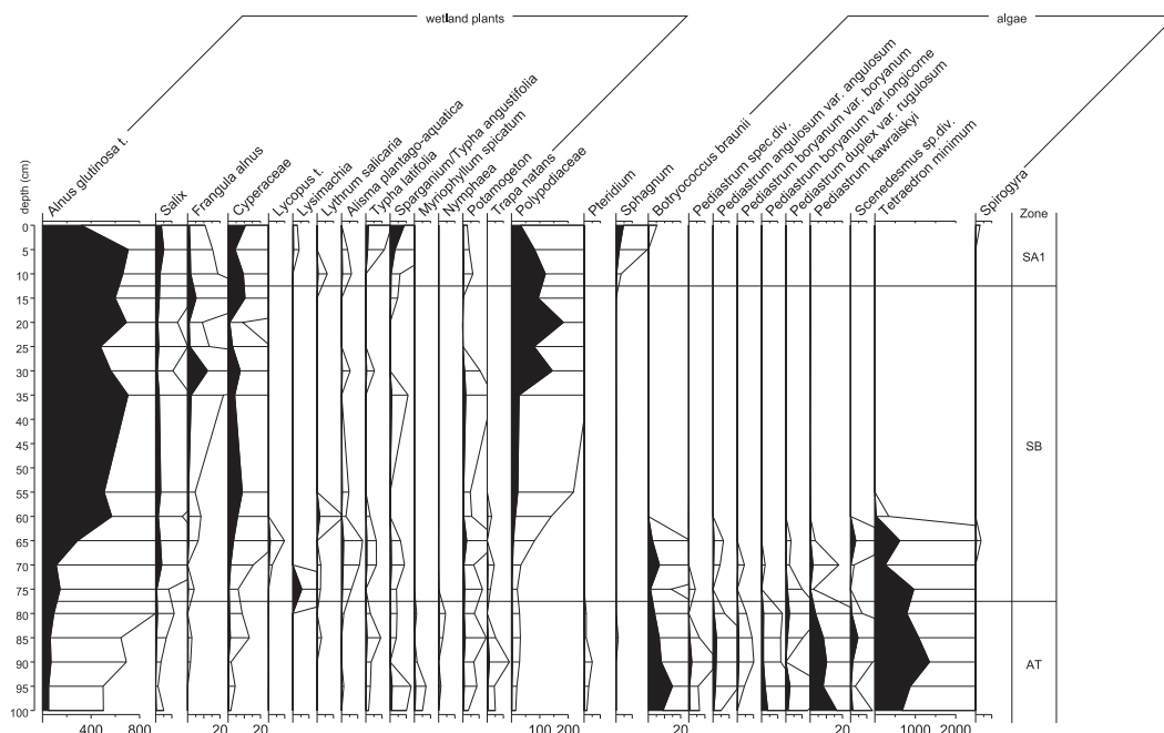
Fig. 6. – Diagram of local pollen and non-pollen objects recorded in the PK-1-D section of the Komořanské jezero lake. Note variable x-axis scales. The analysis was done by Vlasta Jankovská. Percentages of all taxa are related to upland pollen sum.
