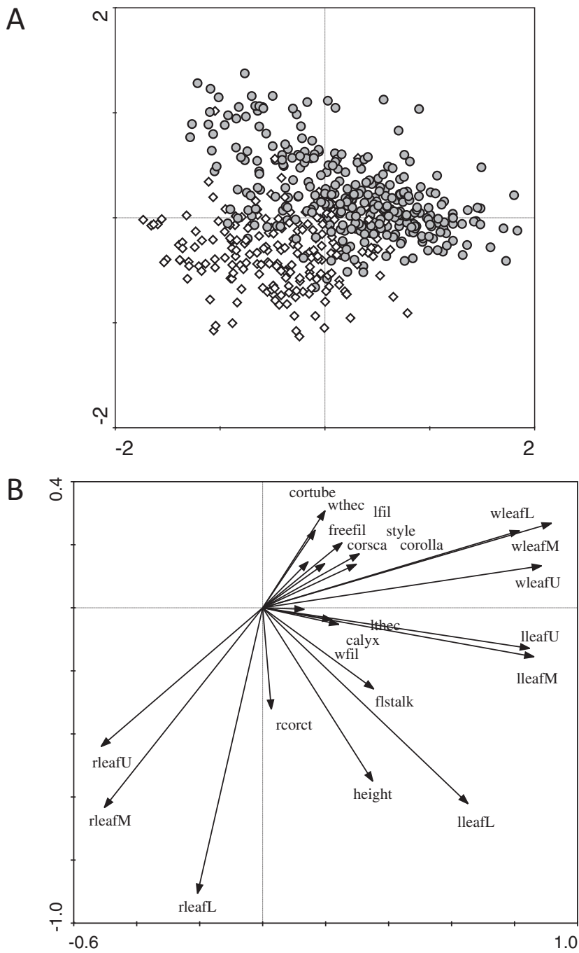
Fig. 7. – PCA of morphological characters of the two cytotypes of Symphytum tuberosum : (A) distribution of individuals in ordination space (◇ 4x, ● 12x), (B) fit of the 18 morphological characters and four ratios studied to the ordination axes (abbreviations of morphological characters explained in Table 1). The first and the second ordination axis explain 48% and 20% of the variation, respectively.
