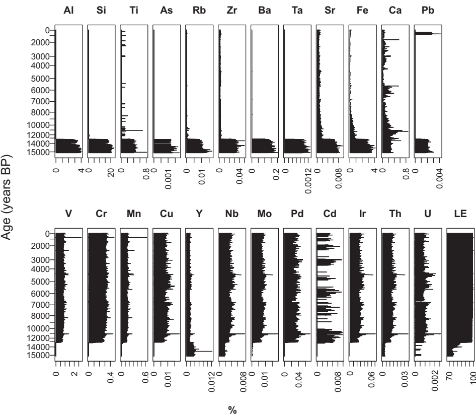
Fig. 3. – Elemental composition of Dárko peat bog sediment, determined using X-ray fluorescence. LE – light elements (from hydrogen to sodium).
