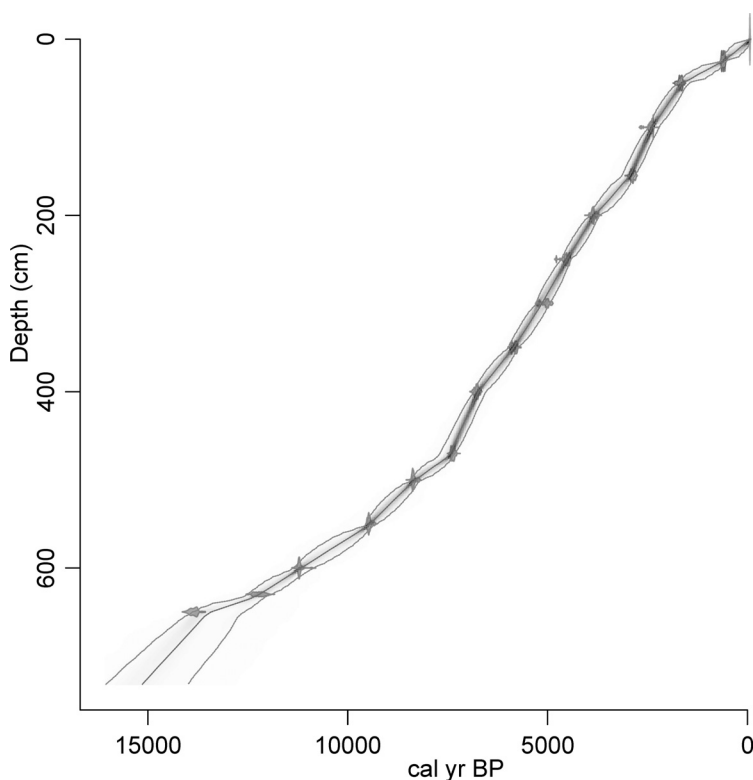
Fig. 2. – Depth-age model of Dárko core: mean value (central dotted line), distributions of calibrated ^{14}\text{C} dates (dark grey polygons) and distributions of modelled ages for all depths (light grey grid). The age between the bottom ^{14}\text{C} date and the base of the core was extrapolated due to the lack of datable material.
