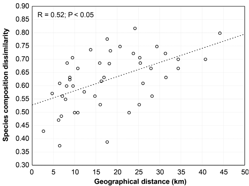
Fig. 5. – The result of the Mantel test; the correlation between species composition dissimilarity and geographical distance matrices for the streams.
