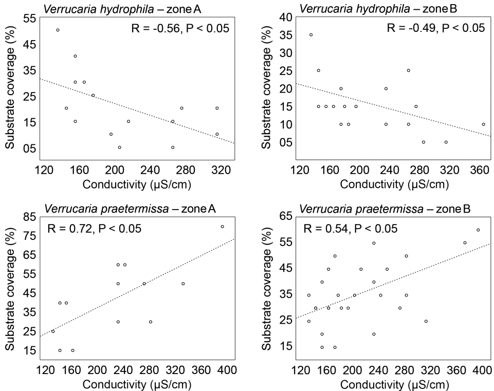
Fig. 7. – Scatterplots showing the relationship between the abundance of lichen thalli at the sampling site (average percentage coverage of 25 cm 2 stone surface by thallus) and conductivity of water measured at this site; Pearson coefficients (R) and P values are provided.
