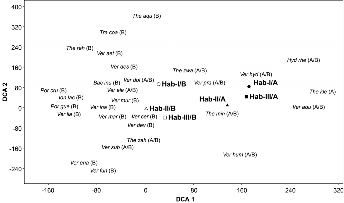
Fig. 6. – Detrended correspondence analysis (DCA) ordination diagram of habitat classes (in relation to hydro-logical zones; Hab-I/A, Hab-II/A, Hab-III/A and Hab-I/B, Hab-II/B, Hab-III/B) and associated species of lichens. The zone (A and/or B) in which a species of lichen was recorded is given in parentheses. See Table 1 for species abbreviations.
