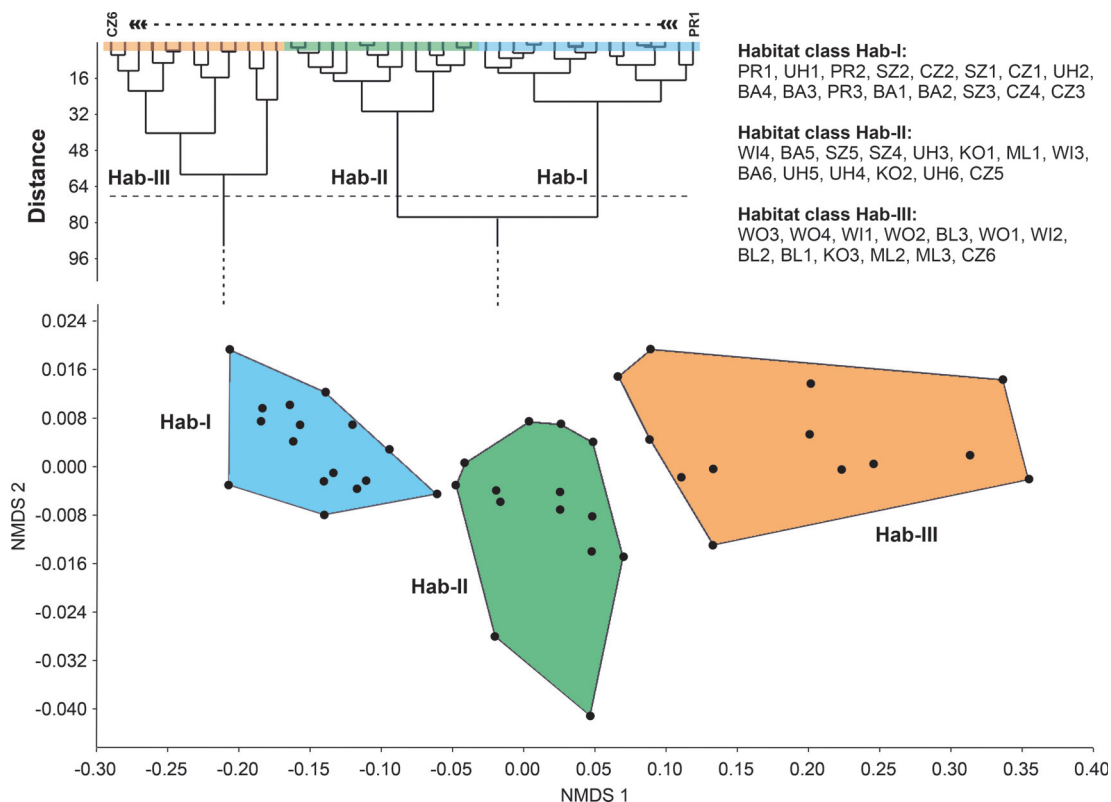
Fig. 1. – Cluster analysis dendrogram (UPGMA) and non-metric multidimensional scaling scatterplot (NMDS) of the sampling sites representing three different habitat classes (Hab-I, Hab-II, Hab-III) separated by pH, conductivity, dissolved oxygen content and silting. The affiliation of sampling sites to a habitat class is provided alongside the dendrogram; sampling sites are listed in order of appearance on the dendrogram. See Material and methods for stream abbreviations and Electronic Appendix 1 for stream locations.
