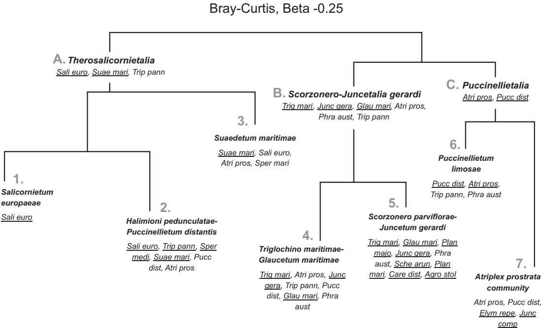
Fig. 2. Classification tree of the cluster analysis. Three higher syntaxa are orders (A, B, C) and seven lower syntaxa are associations (1–7) with abbreviations of their characteristic species. Underlined species are diagnostic, constant and dominant species based on the analysis in JUICE program.
