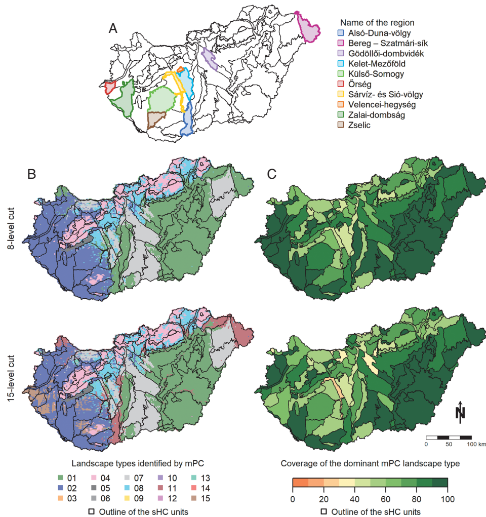
Fig. 5. (A) Location of the regions mentioned in the main text; and (B–C) comparison of the present classification (mPC) at two thematic resolutions (8-group classification – top; 15-group landscape classification – bottom) with that of Molnár et al. 2008 (sHC). In subfigure B, sHC is projected onto mPC. Subfigure C reflects the internal homogeneity of mPC inside each single sHC region based on the percentage cover of the dominant landscape type.
