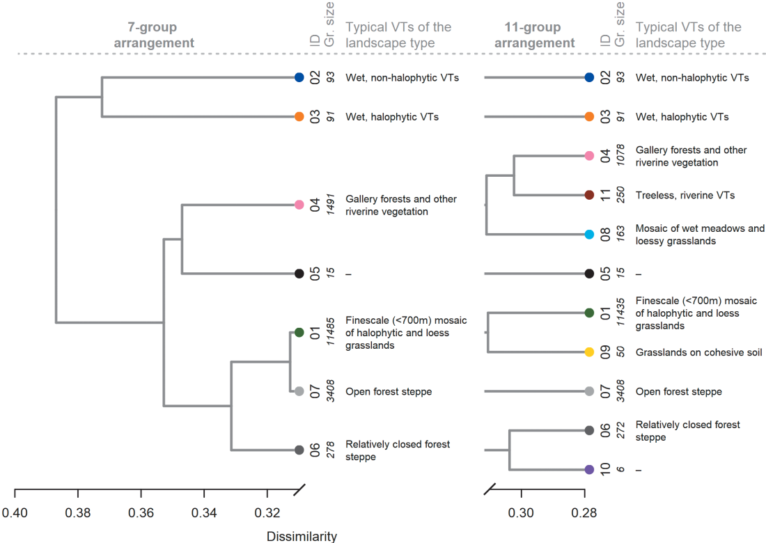
Fig. 6. Dendrogram of the landscape units in the Körös-Maros Interfluvium cut at two levels forming a 7-group (left side) and an 11-group landscape classification (right side). The ID of the group, the number of spatial units it contains (Gr.size) and the dominant vegetation types (VTs) are provided to help with the interpretation at both classification levels. Non-interpretable groups are marked with a dash.
