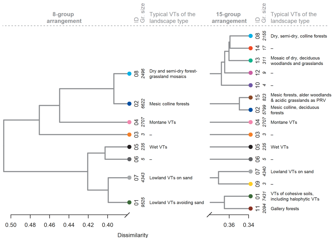
Fig. 3. Dendrogram of the landscape units of Hungary cut at two levels forming an 8-group (left side) and a 15-group landscape classification (right side). The ID of the group, the number of spatial units it contains (Gr.size) and the dominant vegetation types (VTs) are provided to help the interpretation at both classification levels. Non-interpretable groups are marked with a dash.
