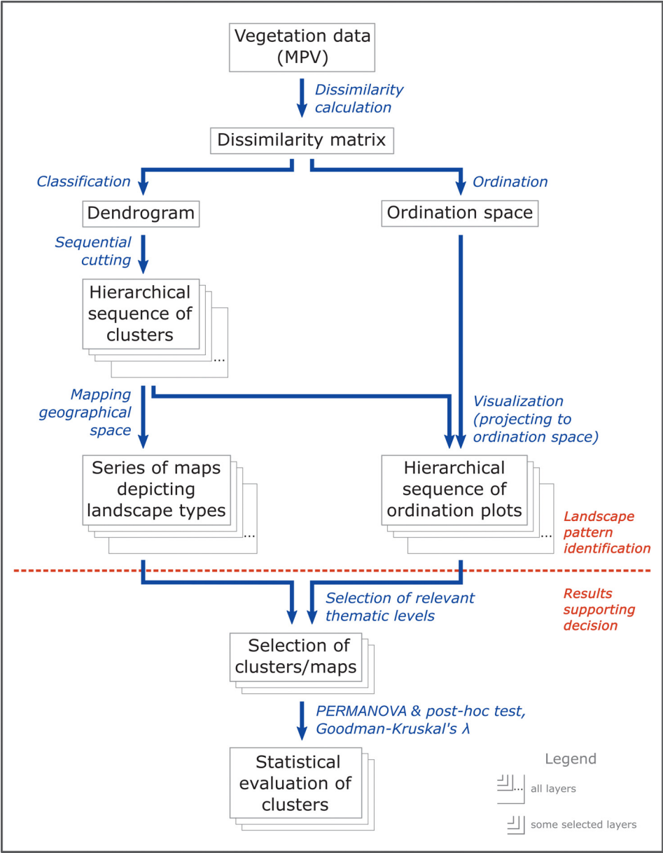
Fig. 2. Conceptual framework of the proposed landscape classification procedure.
