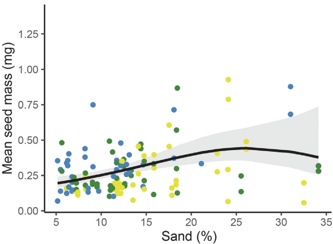
Fig. 6. Relationship between mean seed mass and percentage sand in the sediment. Points show the mean seed mass weighted by the species abundance in 60 plots over two years ( n = 120 ), colours give information on their position on the transverse transect: ● plots nearest the river, ● plots in the middle, ● plots on the top of gravel bars. Regression line shows fit of a generalized linear model (GLM) where the predictors were percentage sand and its quadratic function and the dependent variable was mean seed weight; the grey area shows the 95% confidence interval. Data on seed mass of individual species were obtained from Lososová et al. (2023).
