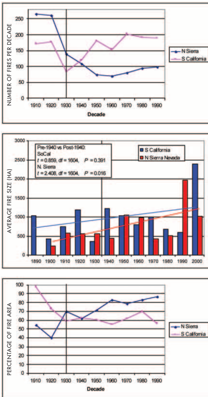
Figure 1. Fire statistics compared between the northern Sierra Nevada (conifer forest) and Southern California (primarily chaparral and non-conifer forest). TOP: Number of fires per decade; MIDDLE: Average fire size per decade; BOTTOM: Percent of the total area burned within a decade contributed by the area of the ten largest fires in that decade. The black vertical line represents the approximate beginning of federal suppression of fires. Source: http://www.frap.cdf.ca.gov/data/frapgisdata/select.asp
