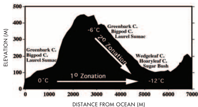
Figure 1. Profile of the change in dominant shrub species of chaparral along a South to North (left to right) transect from the coastal bluffs near Malibu to inland regions near Tapia Park in the Santa Monica Mountains. The transect roughly follows Malibu Canyon Road and the hillsides along this road allow visualization of a vegetation response to this 12^{\circ}\text{C} temperature gradient between the ocean and Tapia Park, approximately 5 km inland (see photograph on page 12).
