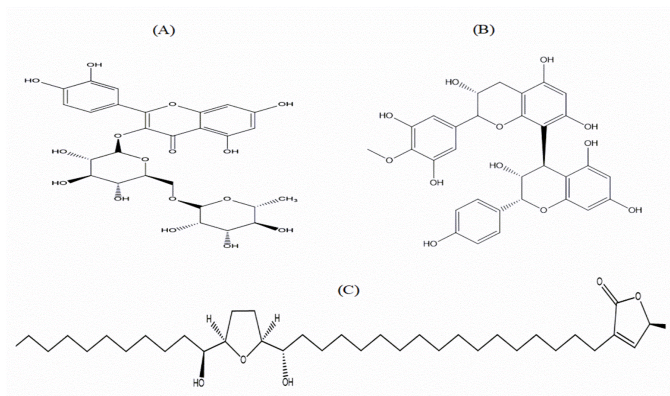
Figure 7. The chemical structure of putative phytomolecules derived from the EEAS. (A) Rutin, (B) Proanthocyanidin, and (C) Squafosacin G chemical structures with their respective molecular formulae: C 27 H 30 O 16 , C 31 H 28 O 12 and C 37 H 68 O 5 .
