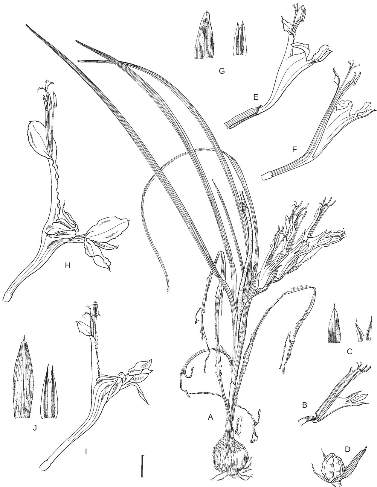
FIGURE 1.—A–D, Babiana avicularis , Goldblatt & Porter 13109 (NBG); E–G, B. hirsuta , Goldblatt & Porter 13110; H, B. ringens subsp. ringens , found at Atlantis, Schnitzler & Manning 13 (NBG); I, J, Babiana ringens subsp. australis , De Waal s.n. (NBG). A, whole plant; B, half-flower; C, outer (left) and inner (right) bracts; D, capsule; E, flower, side view; F, half-flower; G, outer (left) and inner (right) bracts; H, flower; I, flower; J, outer (left) and inner (right) bracts. Scale bar: 10 mm. Artist: John Manning.
