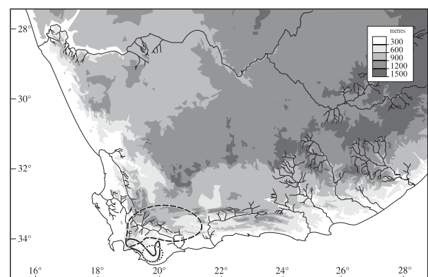
FIGURE 1.—Known distribution of Rhigiophyllum squarrosum (dotted line); Siphocodon spartioides (solid line) and S. debilis (dashed line).
