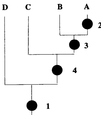
Fig. 5. Alternative cladogram, based on a different interpretation of the data of Fig. 4. Now absence is considered to be apomorphic.
