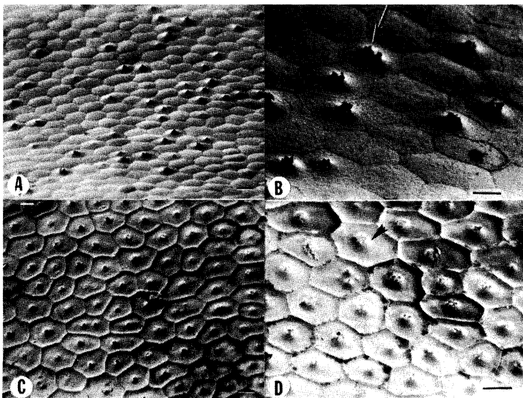
Fig. 1. Scanning electron micrographs of Cyperus compressus achene surface. A,B. Cytotype with n = 56 ; C,D. Cytotype with n = 64 . (Arrowhead = central nodule; Arrow = apical spines. Scale bars = 10\ \mu\text{m} ).
