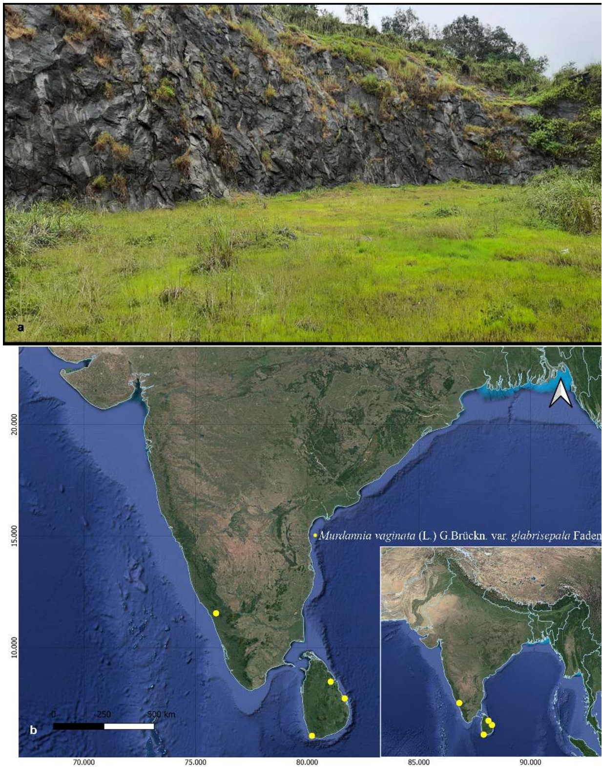
Fig. 4. Murdannia vaginata (L.) G.Brückn. var. glabrisepala Faden: a. Habitat; b. Distribution map, drawn with QGIS ver. 3.28.7 (QGIS, 2023).
