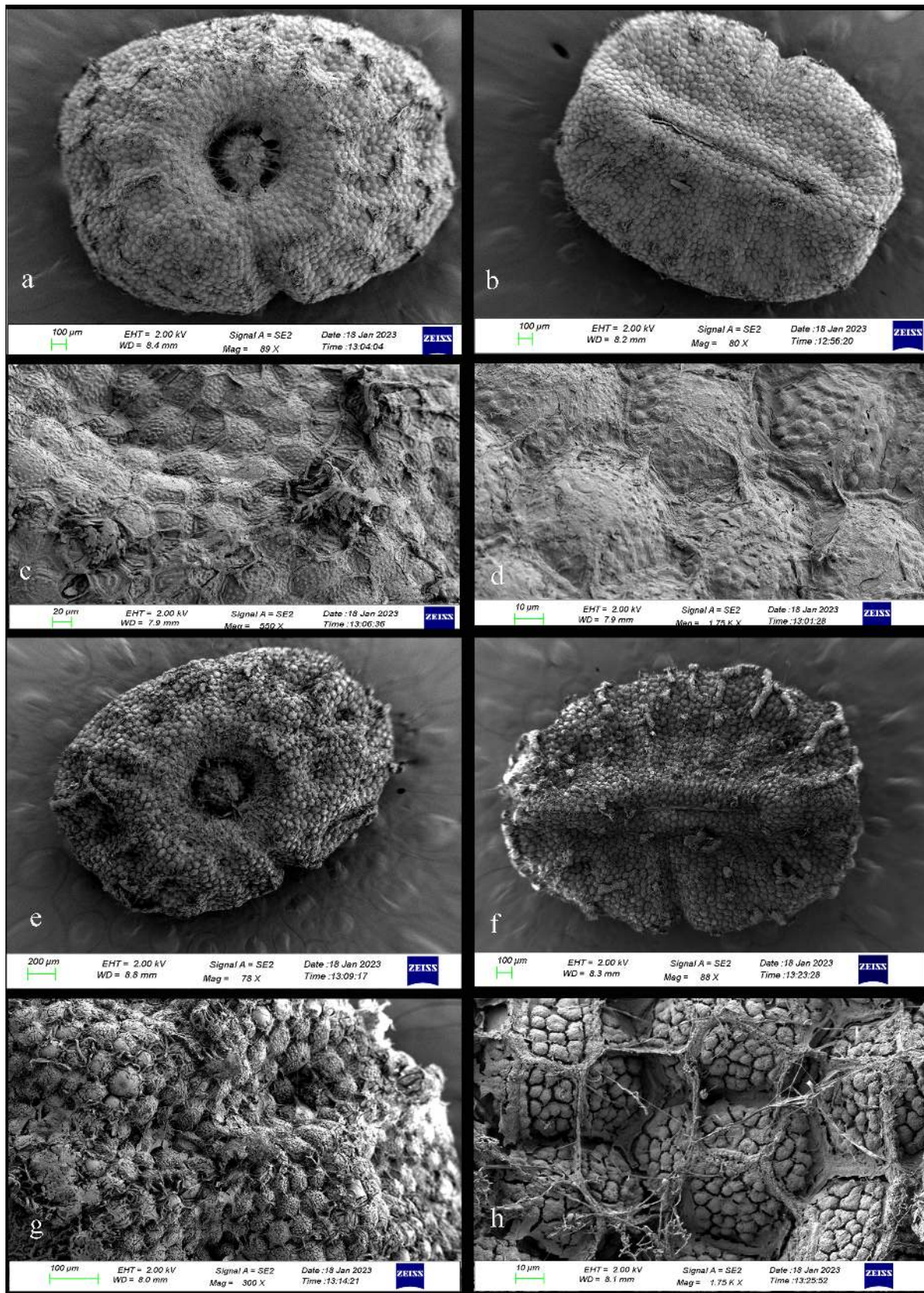
Fig. 2. SEM images of seeds: a–d. Murdannia vaginata (L.) G.Brückn. var. vaginata : a. dorsal view; b. ventral view; c & d. portions enlarged; e–h. M. vaginata (L.) G.Brückn. var. glabrisepala Faden: e. dorsal view; f. ventral view; g & h. portions enlarged.
