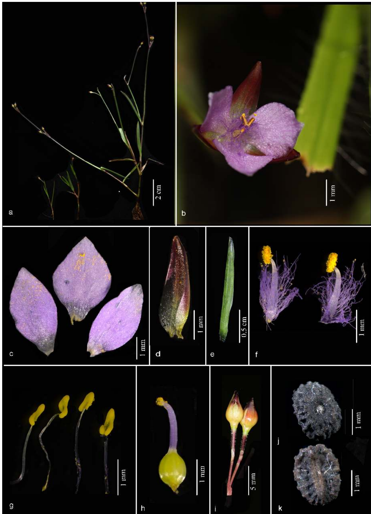
Fig. 3. Murdannia vaginata (L.) G.Brückn. var. glabrisepala Faden: a. Habit; b. Flower; c. Petals; d. Sepal; e. Ribbed sheath; f. Stamens; g. Staminodes; h. Gynoecium; i. Capsules; j. Seed–dorsal view; k. Seed–ventral view (from Sreekutty T.K. & Santhosh Nampy 168000; photos by Sreekutty T.K.).
