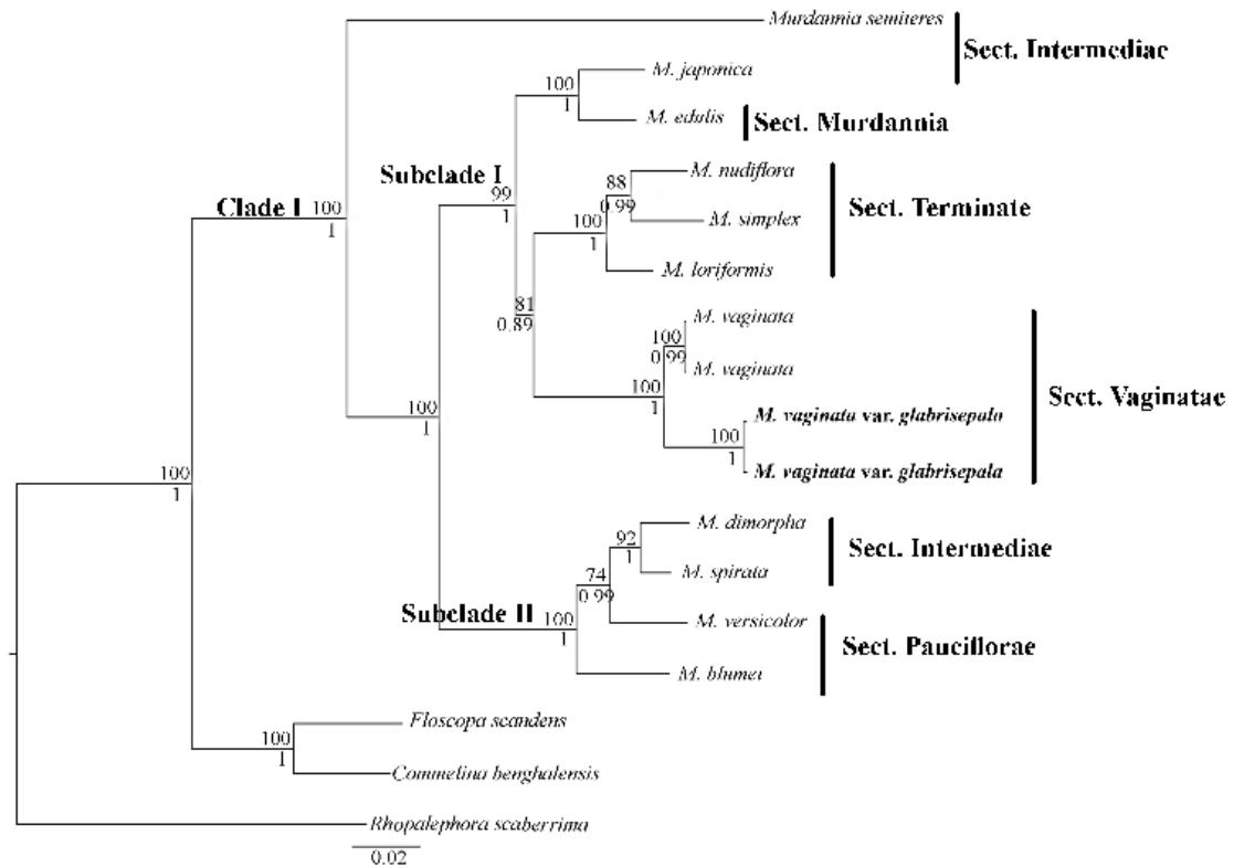
Fig. 1. Maximum Likelihood (ML) phylogram based on combined nrITS, rps16 intron and rbcl gene regions, of 14 Murdannia Royle and three outgroup samples, rooted on Rhopalephora scaberrima (Blume) Faden. ML bootstrap percentages higher than 50% and Bayesian Inference posterior probabilities higher than 0.50 are shown above and below branches, respectively.
