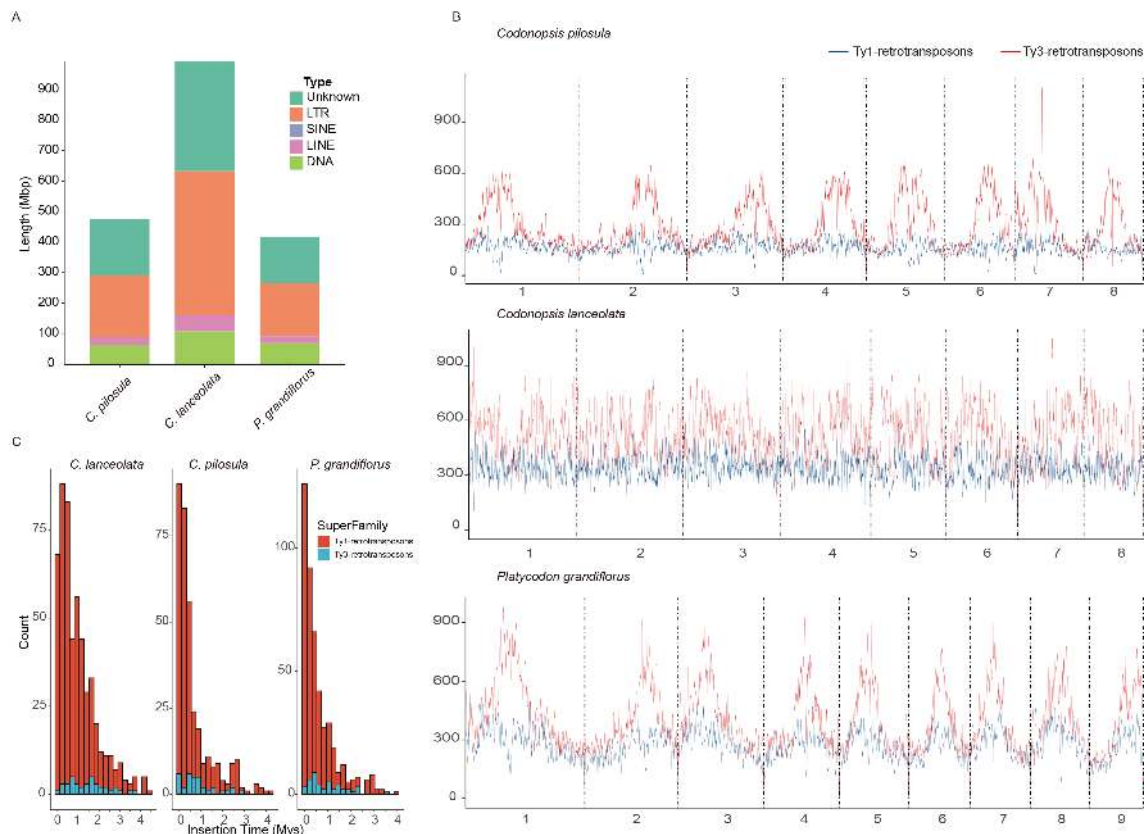
FIGURE 3 Evolutionary analysis of TEs in three platycodonoids species. (A) Sequence size statistics for various types of transposable elements (TEs). (B) LTR density distribution. The Ty1-retrotransposons indicated by a blue line and the Ty3-retrotransposons indicated by a red line. (C) Insertion time distribution of intact Long Terminus Repeat (LTR).
