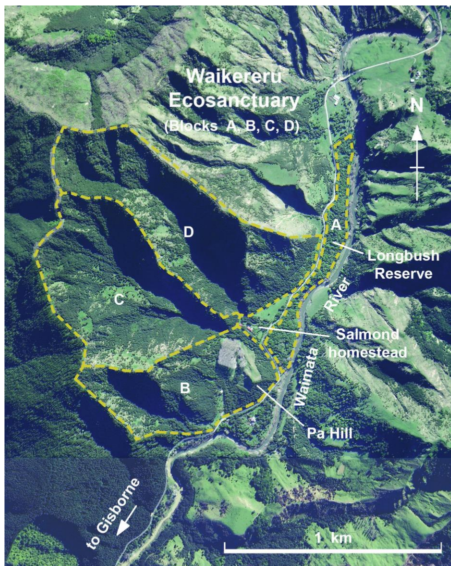
Fig. 3. Vegetation map of Waikereru Ecosanctuary, with the alluvium catchment (A) Long Bush running along the west side of the Waimata river, and separated from the three other hillside catchments (B-D) by the Waimata road (Google maps, 2022, modified by Joshua Salter). Scalebar = 1 km.
