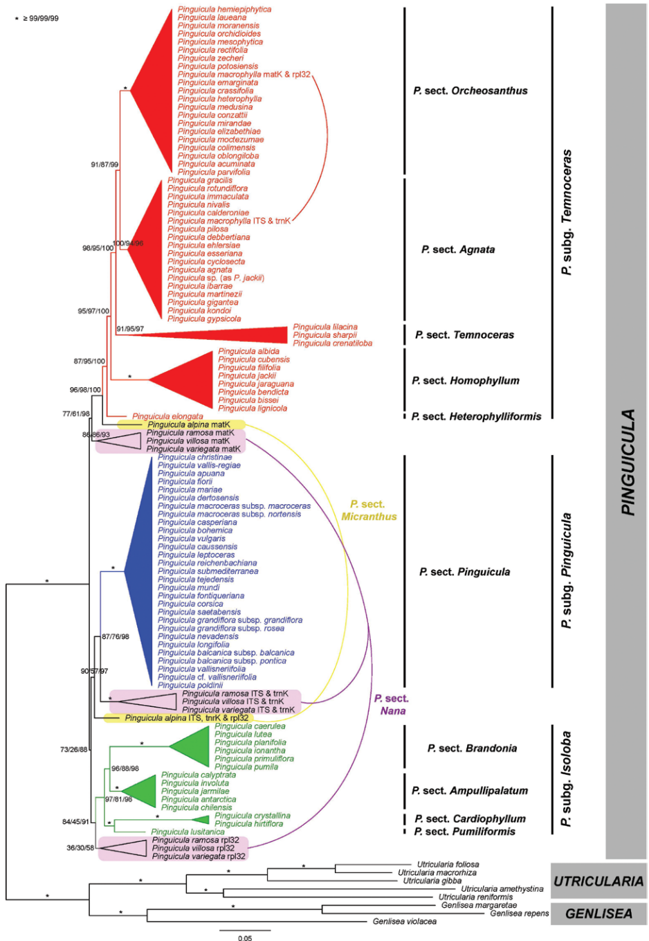
Figure 1: Maximum likelihood phylogram of Pinguicula based on ITS, trnK, matK, and rpl32 DNA sequence data. Numbers on branches denote SH-aLRT/BS/TBE support values. Scale bar represents the average number of substitutions per site.
