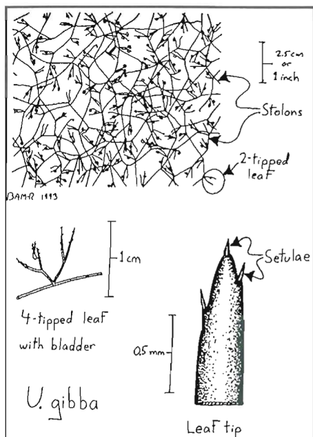
Figure 1: U. gibba —Vegetative features.
