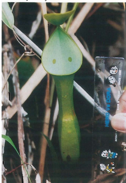
Fig. 3 -- N. reinwardtiana pitcher. Note two "eye dots". Photo by Perry Malouf.
