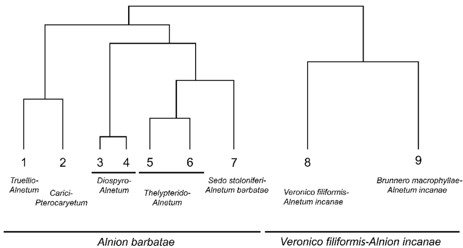
Fig. 5. Dendrogram of the classification analysis ( Beta flexible , Beta = -0.5) of the Caucasian and a Colchic alluvial alder forests and syntaxonomic interpretation of the clusters. For the full names of the abbreviated association names see Methods.
