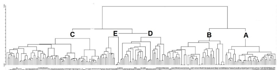
Fig. 3. Dendrogram of relevés with Crambe tataria in Romania. Cluster A – Stipion lessingianae ; Cluster B – Festucion valesiacae ; Cluster C – Cirsio-Brachypodion pinnati and Danthonio-Brachypodion ; Cluster D – Arrhenatherion elatioris ; Cluster E – Prunion fruticosae .
