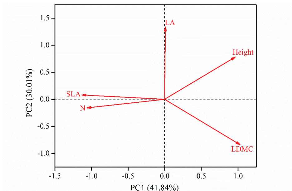
Fig. 5. PCA ordination to present the covariance amongst the studied functional traits of the vegetation. Eigenvalues for 1st and 2nd axis: 2.09 and 1.50, respectively; explained variation: 41.8 % and 30.0 %, respectively. LDMC = leaf dry matter content, LA = leaf area, SLA = specific leaf area, N = shoot nitrogen content, Height = shoot height.
