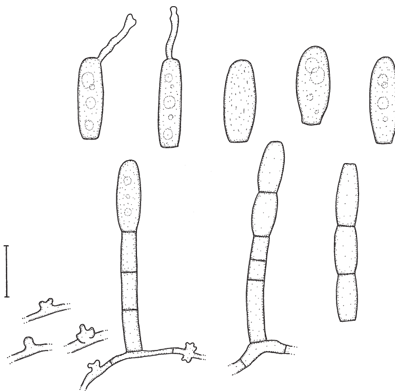
Fig. 1: Oidium jacarandigena sp. nov., conidia, conidiophores, appressoria; scale = 20 µm; U. Braun del.
