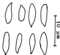
Sporen
