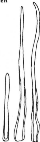
Sporen
