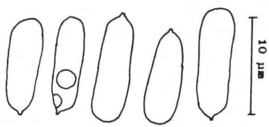
Sporen
