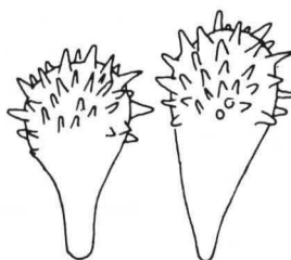
Sporen
