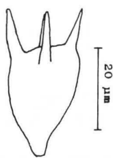
Basidie
