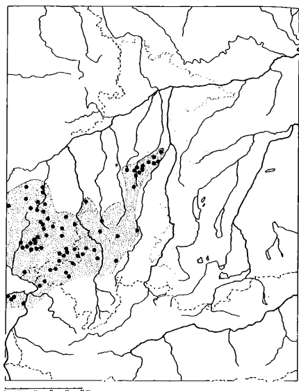
Alnus viridis
