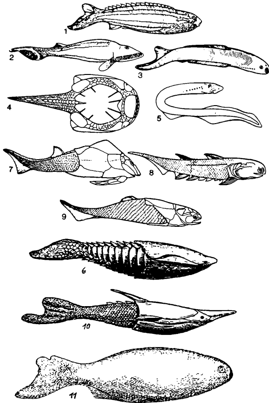
Abb. 3 Vertreter der Agnathi (1 - 4, 6, 10, 11), Cyclostomen (5), Placodermi (7, 9), Acanthodi (8).
