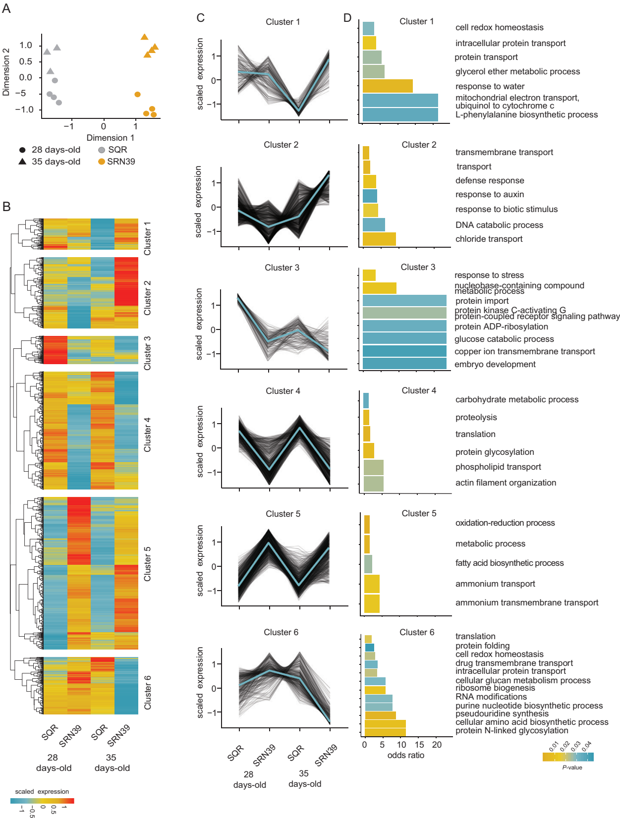
Fig. 1. Transcriptome profiles of roots of Shanqui Red (SQR) and SRN39. (A) Multidimensional scaling plot of samples based on their transcript abundances (log 2 counts per million, CPM). Gray, SQR; orange, SRN39; circles, 28 d old; triangles, 35 d old. (B, C) Six clusters of genes affected by a
